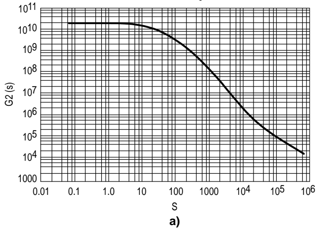
Figure 18. a) Simulated Double-Pole Bode Plot of System, and b) Simulated Phase Angle Double-Pole System
