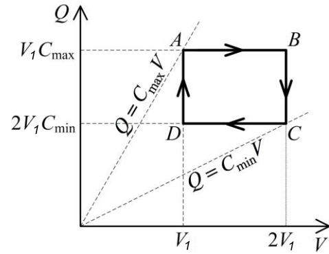
Fig. 2. QV-diagram of the harvesting cycle when V_1 = V_{init} : AB and CD: diodes are blocked, DA: D_1 is ON, BC: D_3 is ON.
