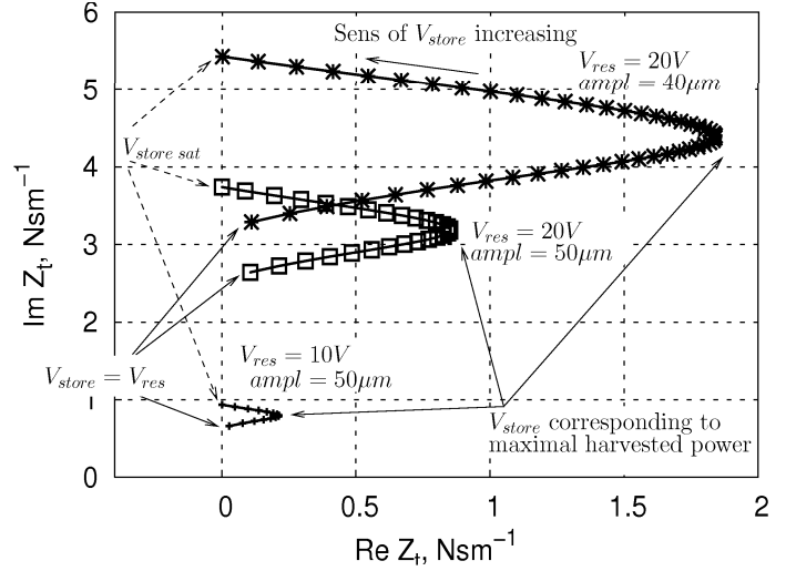
Figure 4: Evolution of the transducer impedance during the charge pump operation.
